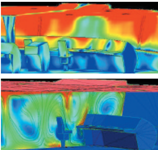
CFD technology simulating air flows on the bridge
