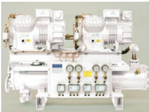
Semi-hermetic condensing unit
